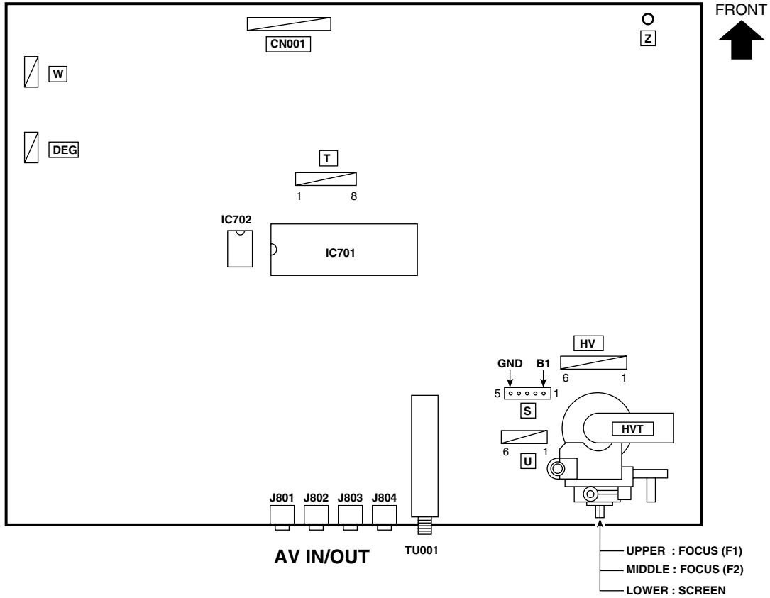
MAIN PWB
