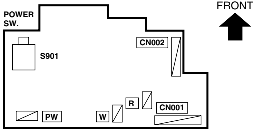
FRONT CONTROL PWB(1/2)
