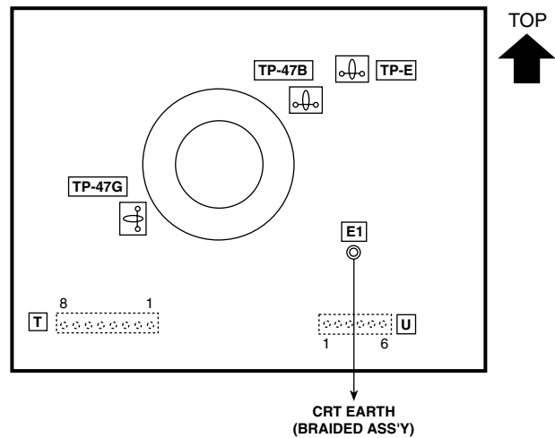
CRT SOCKET PWB (SOLDER SIDE)
